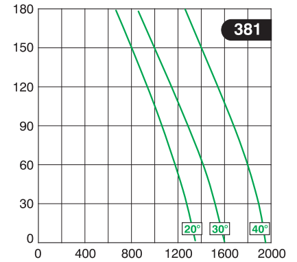
Airflow (L/s)
